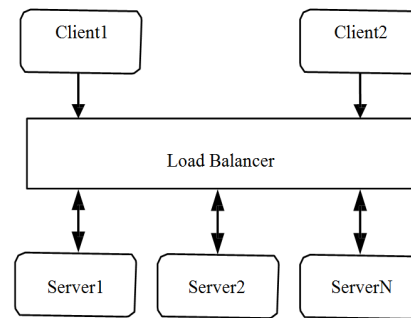
Figure. 1. Load balancer
