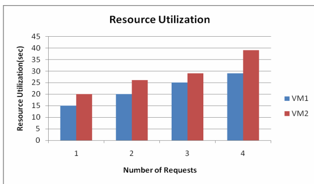
Figure. 9. Resource Utilization
