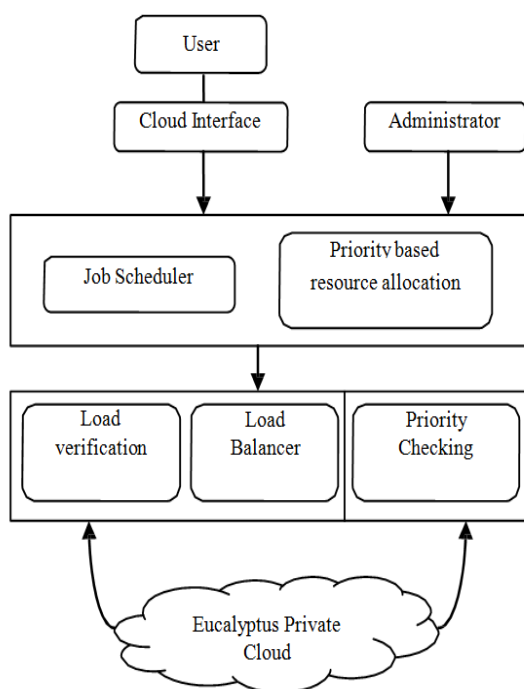
Figure. 2. Cloud Architecture
