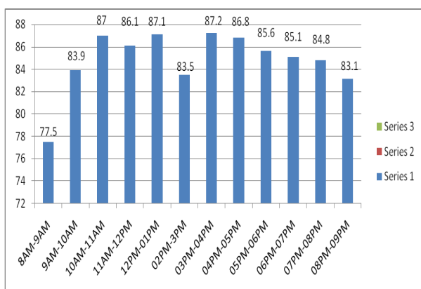
Figure 8: Temporal distribution of equivalent noise level Leq dB GOHALPUR
