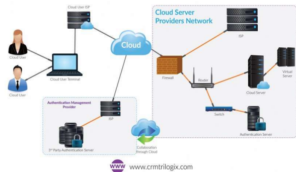
Figure 1. Framework of Proposed CAM System
