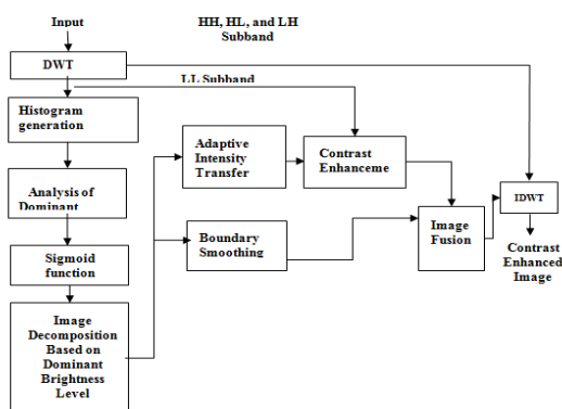
Figure 1: Block Diagram
