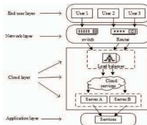
Figure 2. Load balancing in cloud computing
