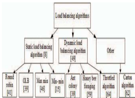
Figure 3. Classification of load balancing algorithms.
