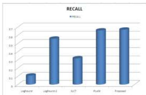
Figure 2: Value of Recall for various algorithms
