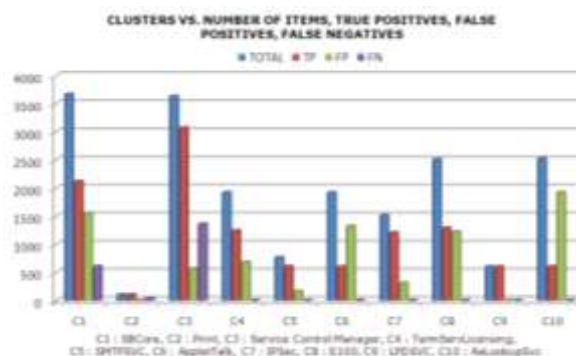
Figure 5: Frequency of items in each Clusters
