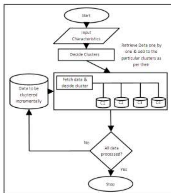
Figure 1: Flow Chart indicating the flow of processing to be done for implementation of the proposed algorithm
